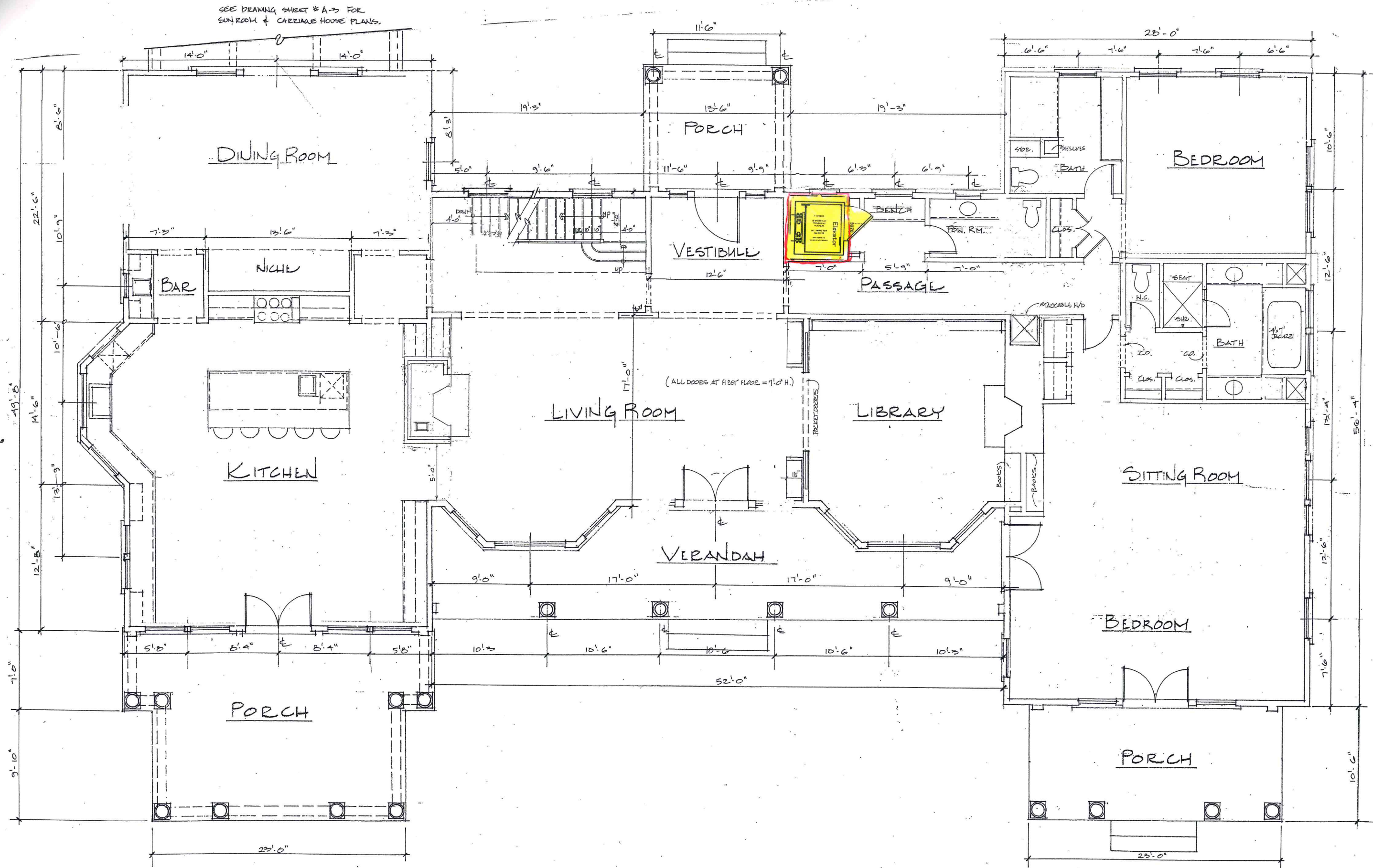
PROPOSED FIRST FLOOR PLAN AT MAIN HOUSE
